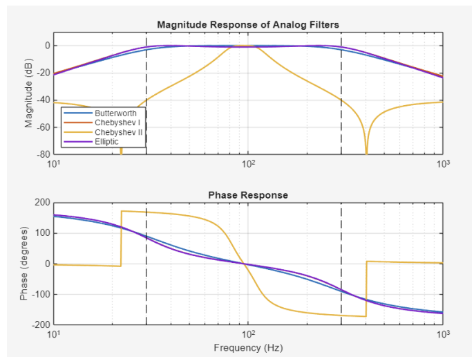
Figure 14. Bode Plot for Butterworth, Chebyshev I, Chebyshev II, and Elliptic Filters.
