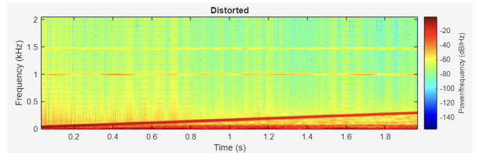
Figure 7. Distorted Signal y(t) Spectrogram Frequency Sweep.
