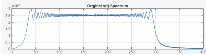
Figure 3. Magnitude Spectrum of the Original Signal x(t) .
