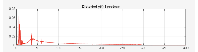
Figure 6. Magnitude Spectrum of the Distorted Signal y(t) .
